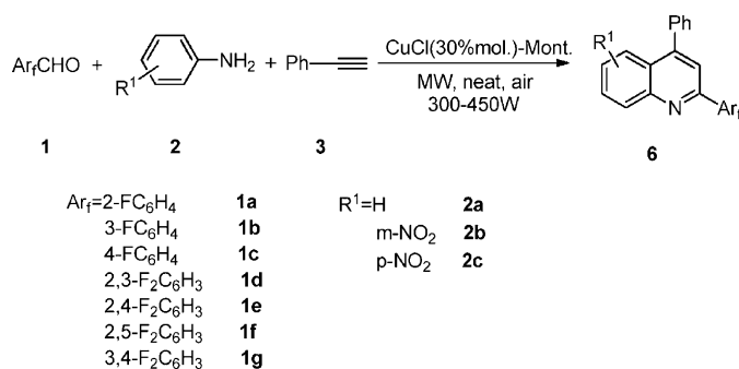
Scheme 3. Synthesis of quinoline derivatives 6.
