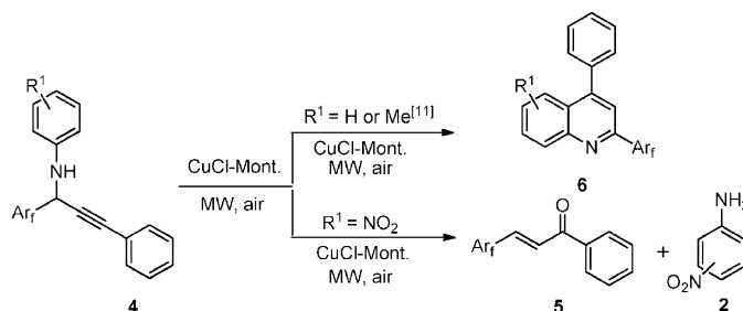
Scheme 2. Chemical transformation of 4 to 5 or 6.
